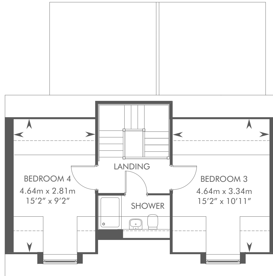
SECOND FLOOR
